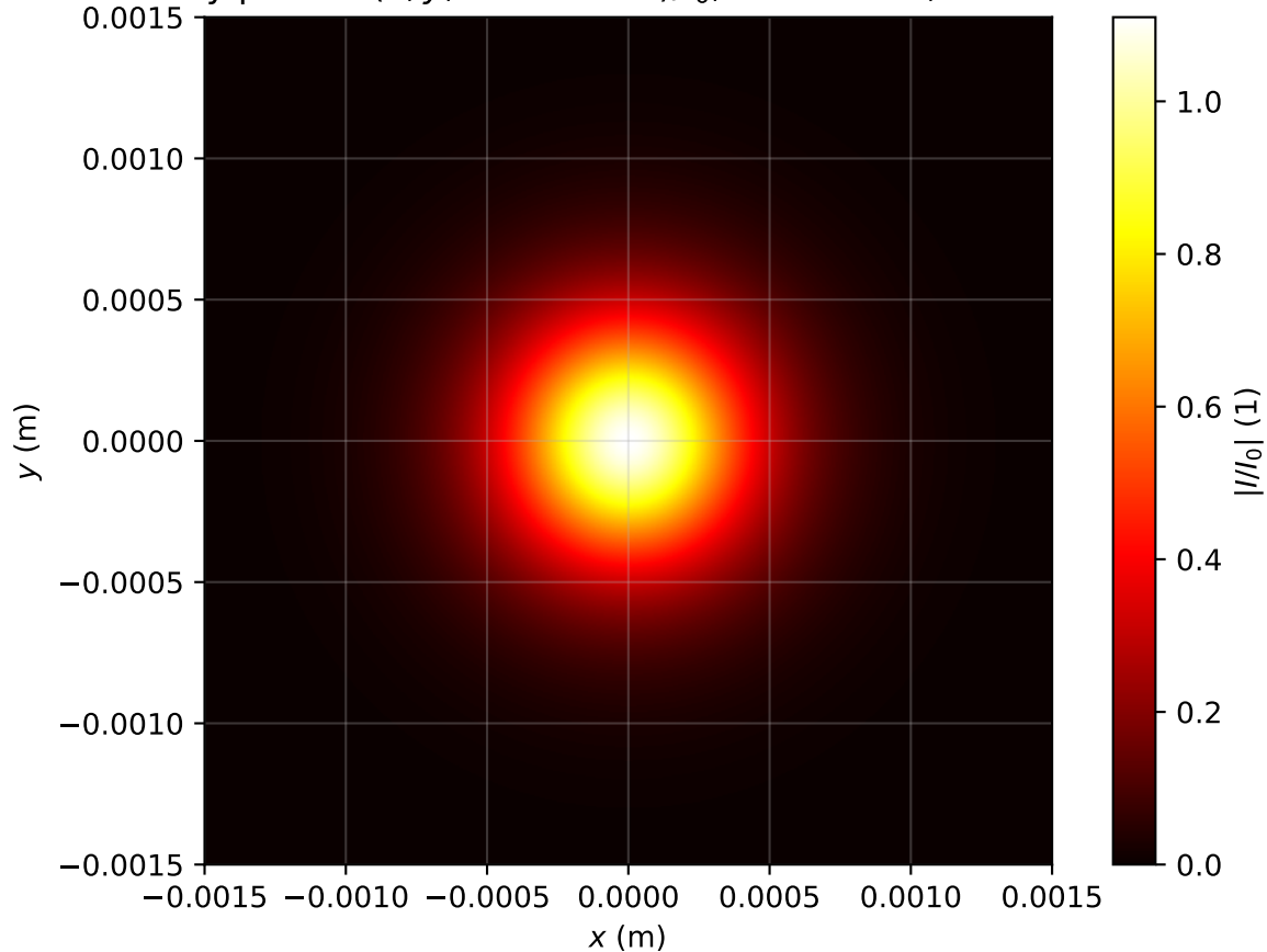
Intensity profile I(x, y, z = 1.194m)/I_0 , P_{in}=0.6P_{cr} , artificial time
